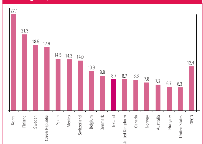
Figure 4.1 Engineering degrees 78 as a percentage of total new degrees, 2005
